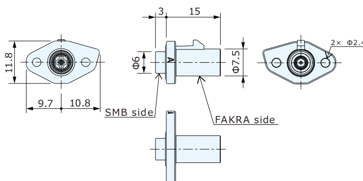
変換アダプタ：CKV9001-02□□F
