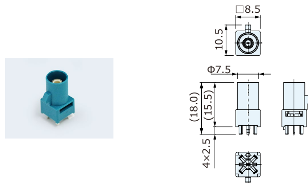
基板用Plug CRC5001-64□□F
